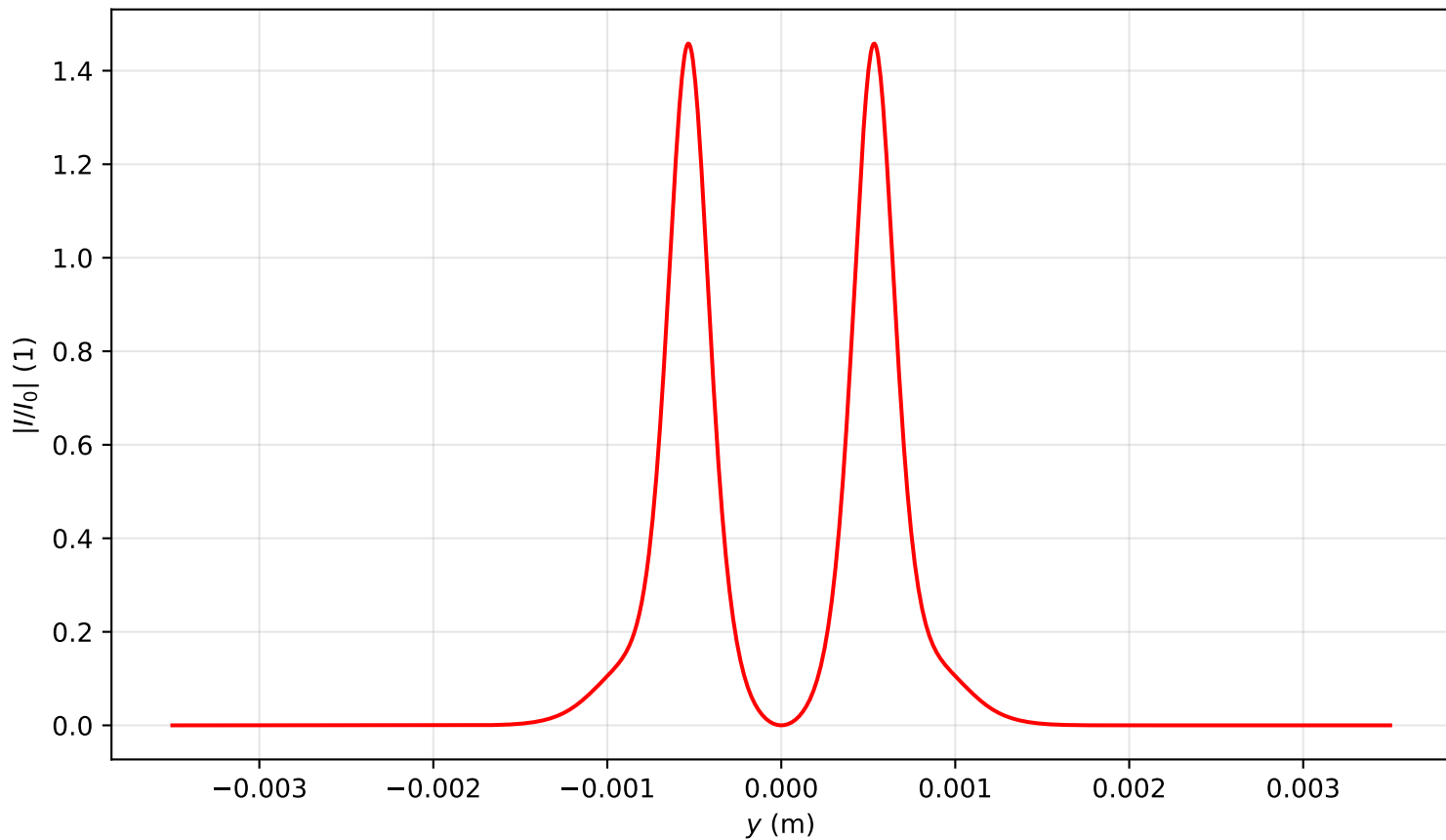
Intensity profile I(x=0, y, z=0.557)/I_0 , P_{in}=7.0P_{cr} , artificial time
